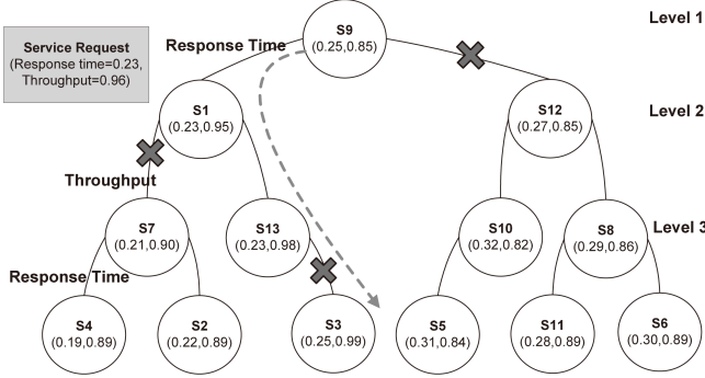
Figure 2: K-d tree example
