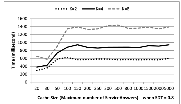
Figure 6: Computation time with different cache size
