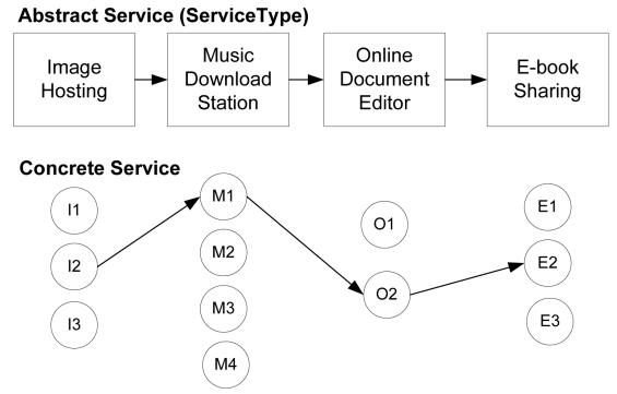
Figure 1: Atomic service selection
