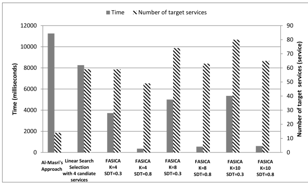
Figure 4: Comparison with other approaches
