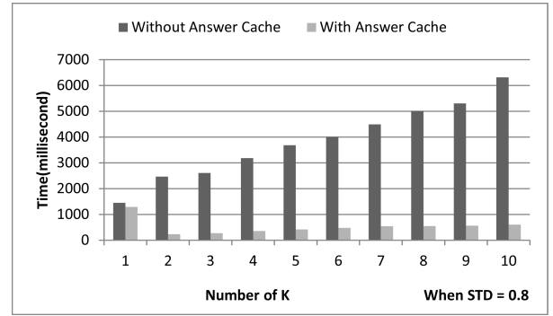
Figure 5: Computation time with and without Answer Cache
