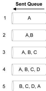
Figure 3: Sent Queue
