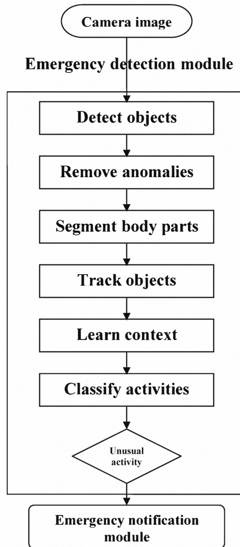
Fig. 1: Flowchart for the emergency detection module.
