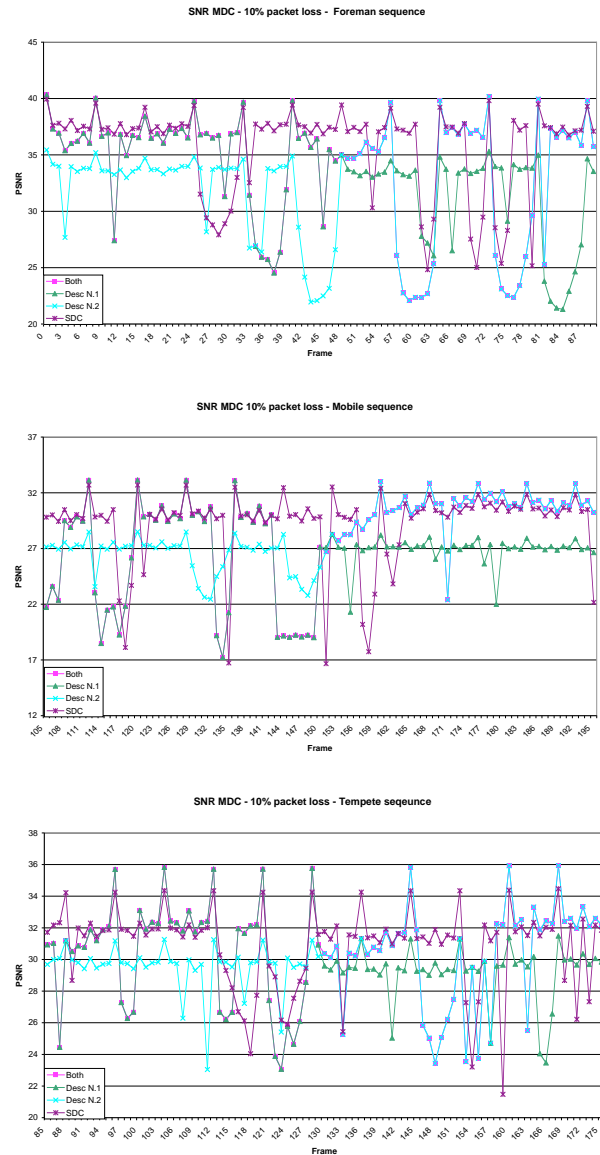
Figure 7 Performance of the SNR MDC algorithm with 10% losses.
