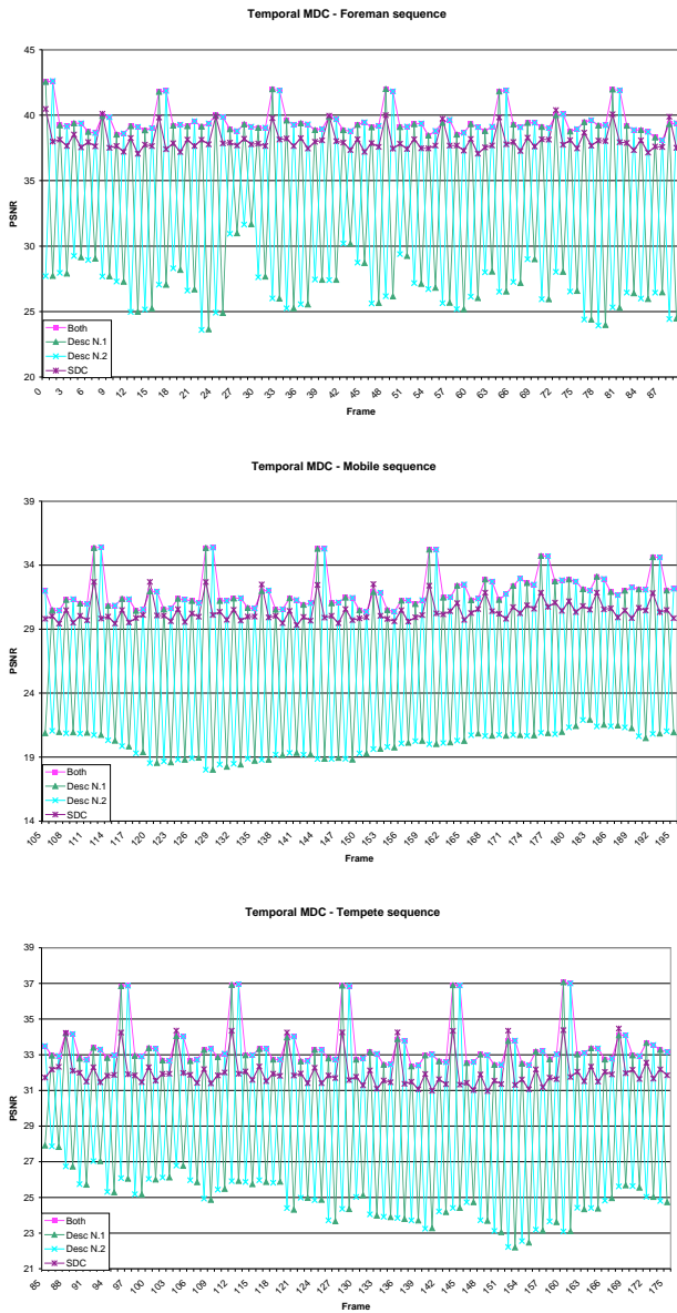
Figure 4. Performance of the temporal MDC algorithm without losses
