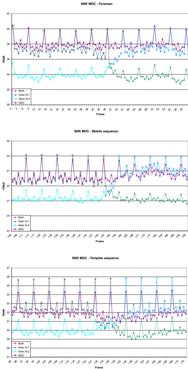
Figure 6 Performance of the SNR MDC algorithm without losses.
