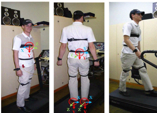
Figure 1. Accelerometer sensors placement and axis orientation
