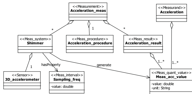
Figure 3: Example of the domain-specific ontology that defines the measurement of acceleration.
