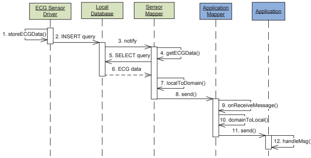
Figure 4: Example of data sharing between the sensor driver and the application via ontology mappers.
