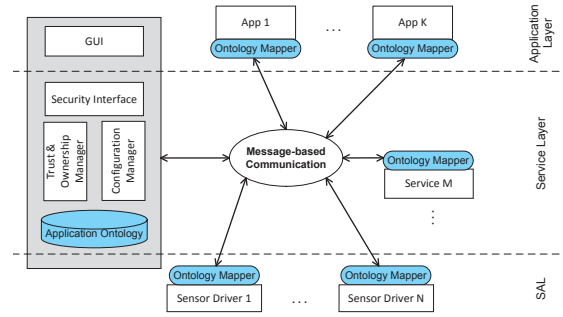
Figure 5: The architecture with decentralized data stores (local data stores are not shown).
