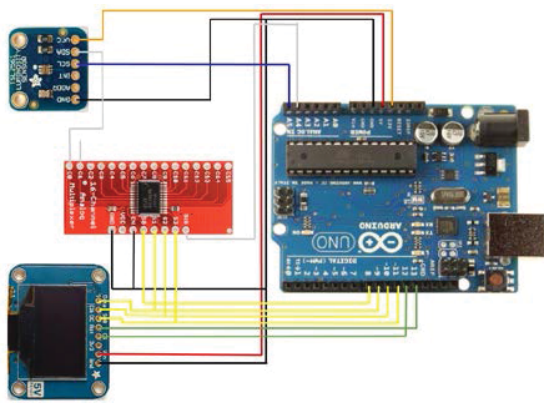
Figure 2. Layout of the component connection and wiring for a single light sensor, with images of hardware components, including TSL2561 light sensor, 4x16 mux, Arduino Uno microprocessor, and 128x64 OLED display.
