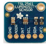
Figure 1. Image of TSL Light Sensor with broadband (top left circle) and infrared (top right circle) photodiode.
