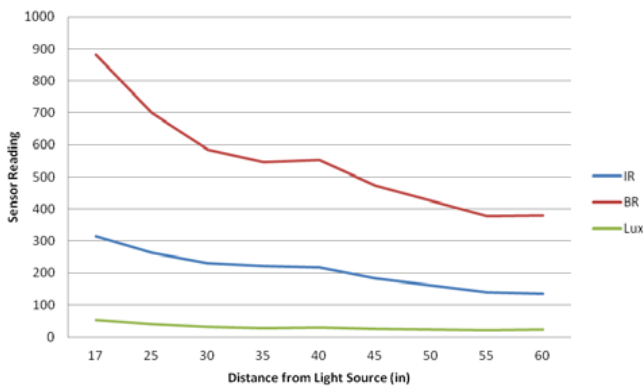
Figure 8. Infrared (IR), Broadband (BR), and lux values variation, with the increase of the light source distance from 17 to 60 inches.
