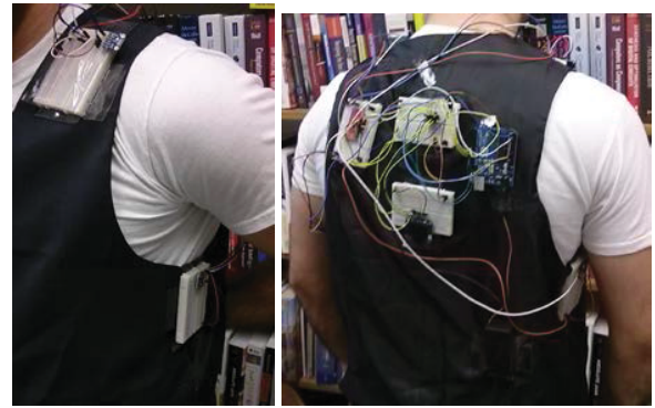
Figure 4. Image of LightVest, including Arduino Uno microprocessor and four light panels from front and back.
