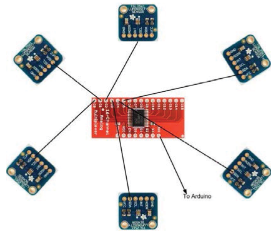
Figure 7. Figure of placement of the light sensors, to determine direction of light.
