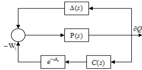
Figure 6. The control system feedback AQM
