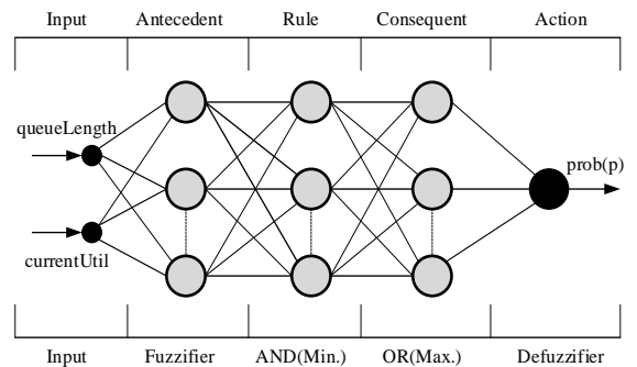
Figure 10. Architecture of FNNREM
