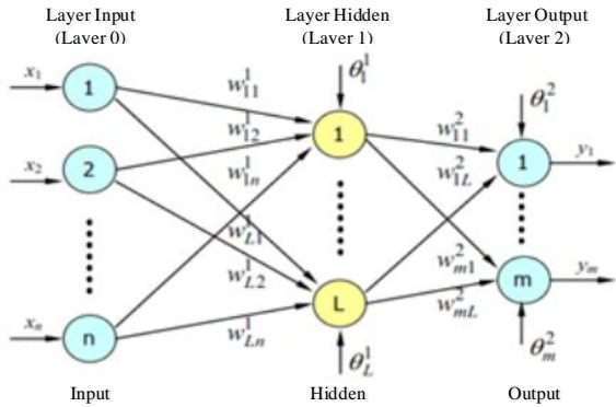
Figure 8. System 2-layer feed forward neural networks
