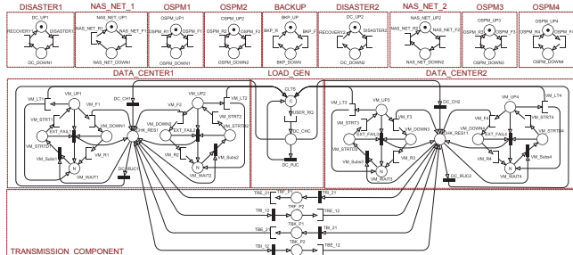
Figure 3: Reliability model of a cloud architecture
