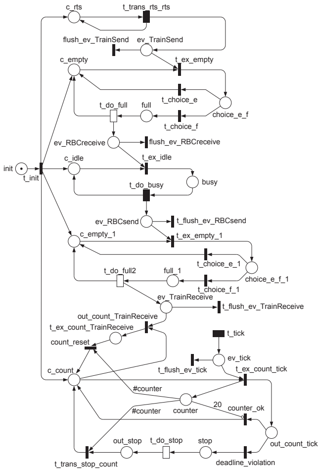
Figure 2: Stochastic Petri net of ETCS communication and control message timeouts
