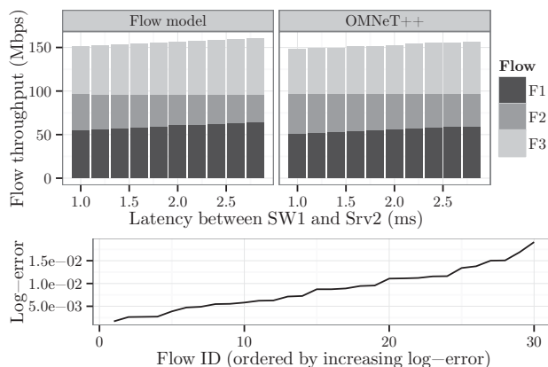
Figure 10: Comparison between the flow model and the OMNeT++ results for the dumbbell topology with cross-traffic (see Figure 8) with the improved model taking into account TCP ACKs, with the bandwidth (above) and the log-error (below)
