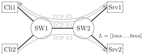
Figure 8: Dumbbell topology with cross-traffic
