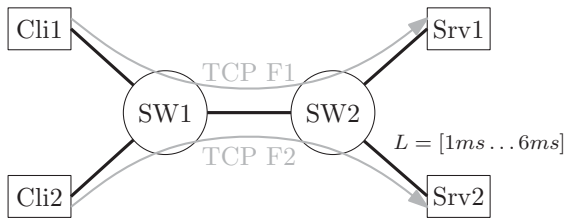
Figure 6: Dumbbell topology without cross-traffic
