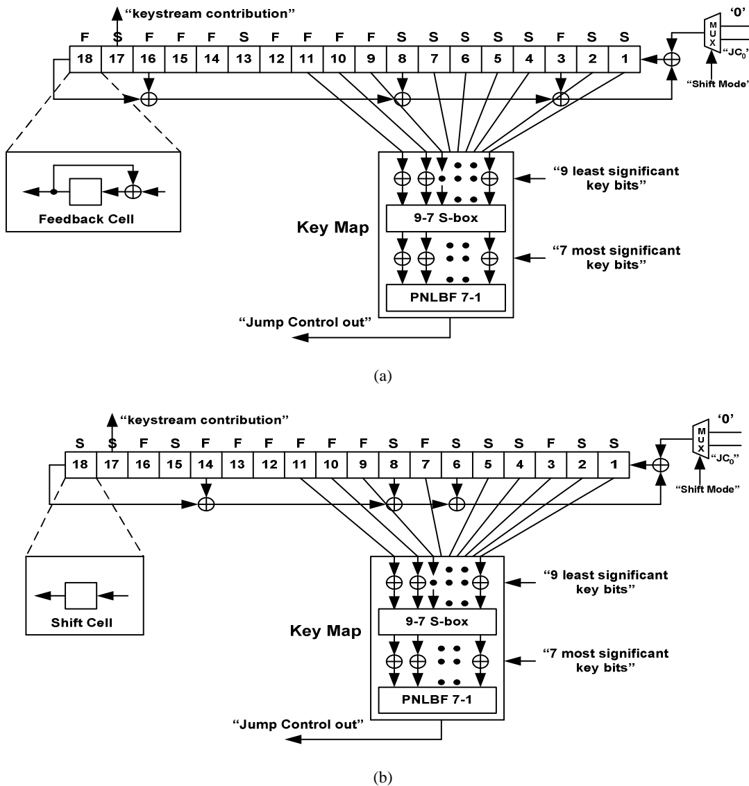
Figure 2. Jump Register Section (a) Type 1 (b) Type 2.
