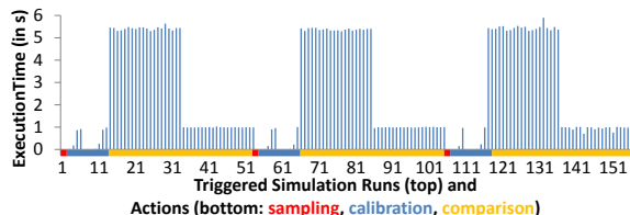
Figure 7: The first actions and corresponding simulation runs executed for the example in Figure 6.
