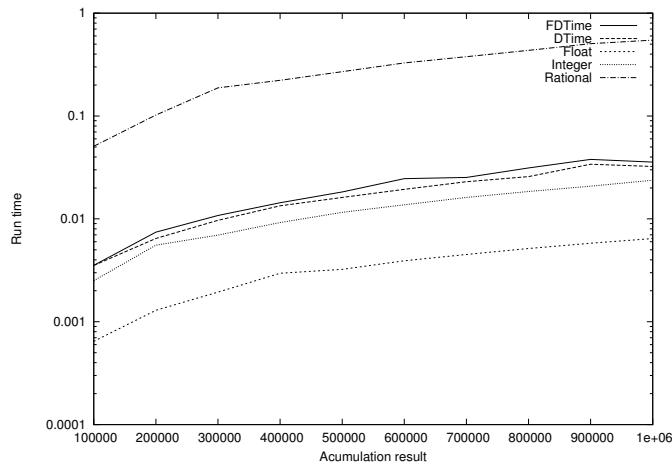
Figure 1: Series y = 1 with no compiler optimization.
