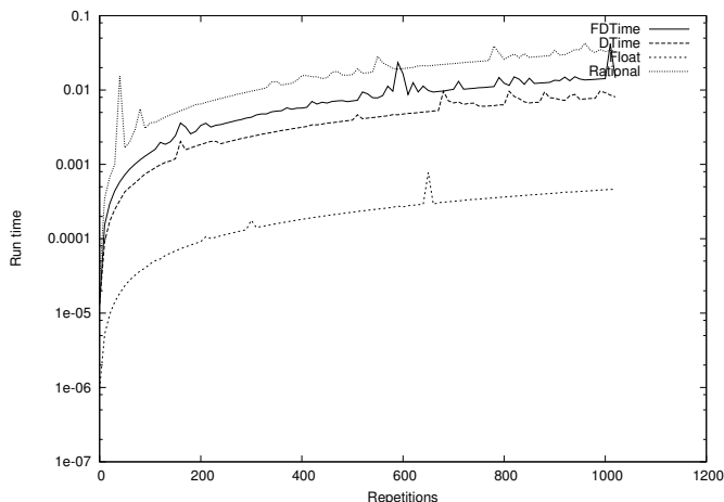
Figure 5: Series y = 1/2^x with no compiler optimization.
