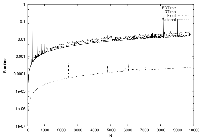
Figure 7: Series y = 1/p_i where p_i is the i -esieme prime with no compiler optimization.
