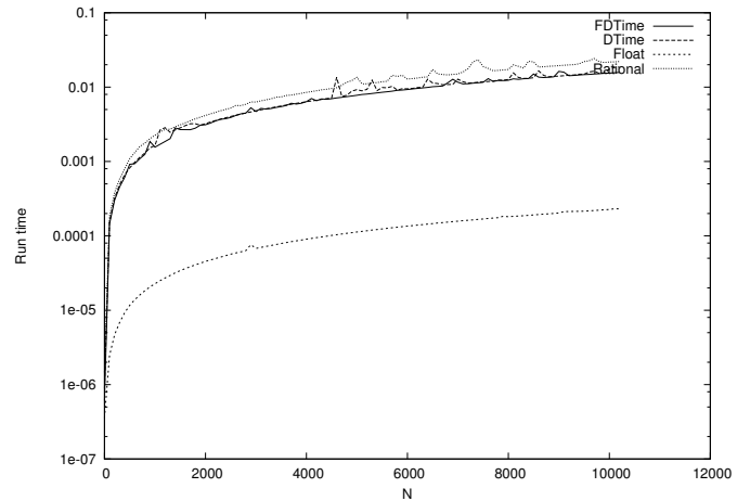
Figure 3: Series y = 1/x with no compiler optimization.
