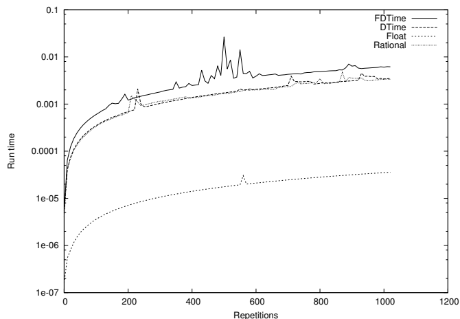
Figure 6: Series y = 1/2^x with -O2 compiler optimization.
