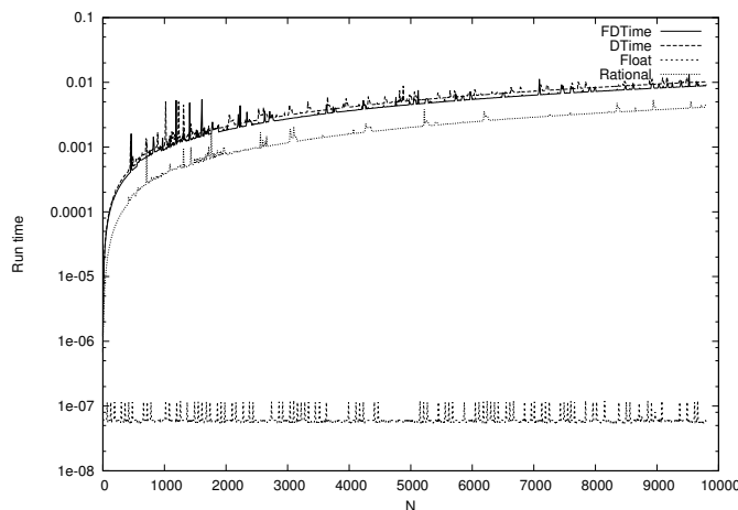
Figure 8: Series y = 1/p_i where p_i is the i -esieme prime with -O2 compiler optimization.
