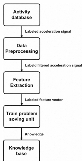
Fig. 3. Principal process of creating a knowledge base for knowledge-based methods for the purpose of posture and activity recognition.
