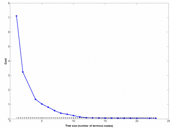
Fig. 4. Cost of nodes of the decision tree. The cost of a node is the mean squared error over the observations in that node.
