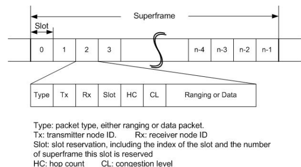
Figure 2. Data channel structure
