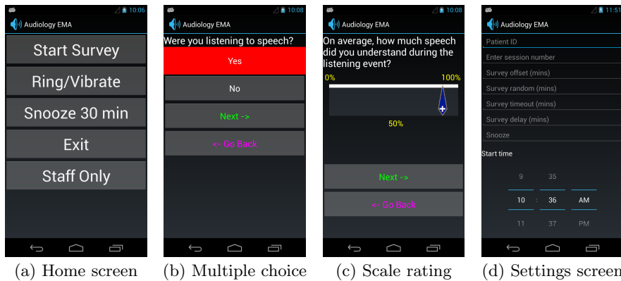
Figure 1: AudioSense mobile application
