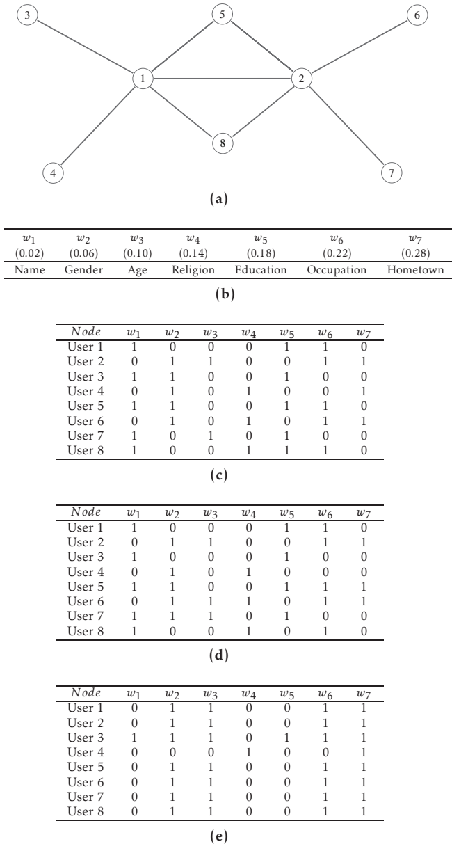
Figure 3. (a) A sample network consisting of 8 users connected to each other, (b) each user has a profile with 7 attributes with a weight vector (w_1, w_2, \dots, w_7) = (0.02, 0.06, 0.10, 0.14, 0.18, 0.22, 0.28) , (c) initial sign flags for all 8 users that indicate which attributes are revealed and which attributes are withheld (a "1" indicates an attribute revealed while a "0" indicates an attribute withheld), (d) after every user compares his strategy with that of his neighbors, every user updates their strategy, (e) the illustrated system converges after 11 iterations and gives the resultant sign flags for all users.
