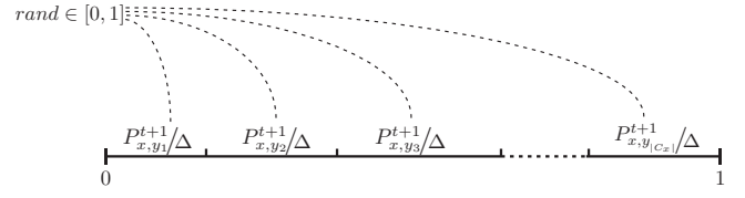
Figure 2. The figure shows the implementation of selecting one of the candidate neighbors as y^* based on the model of balls into non-uniform bins , where C_x = y_1, y_2, \dots, y_{|C_x|} . The probability of selecting neighbor y_i is directly proportional to P_{x,y_i}^{t+1}
