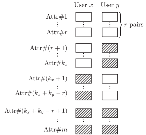
Figure 1. The figure shows a possible profile configuration for two users x and y , who disclose k_x and k_y attributes respectively out of the m possible attributes. The clear rectangles represent the disclosed attributes while the shaded rectangles represent withheld attributes.
