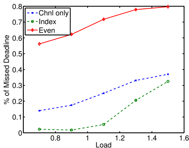
Figure 5. Percentage of Jobs Missed Deadline when Index Policy Objective is Minimizing Missed Deadlines, Synthetic Trace
