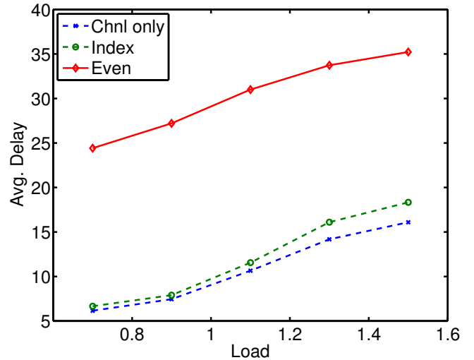
Figure 6. Average Delay when Index Policy Objective is Minimizing Missed Deadlines, Synthetic Trace
