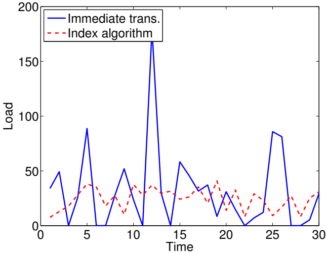
Figure 4. Traffic smoothing
