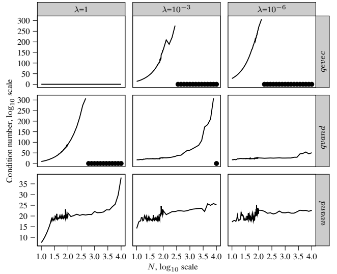
Figure 3: Condition number.
