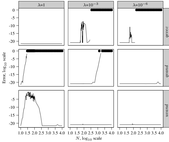
Figure 2: Error.
