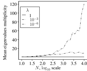
Figure 7: Mean eigenvalues multiplicity.
