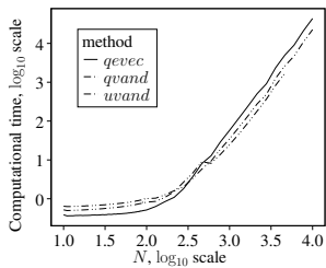
Figure 6: Computational time.
