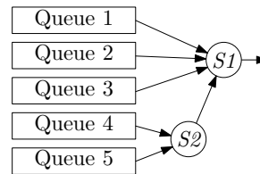
Figure 2: Example of hierarchical scheduling with two schedulers S1 and S2
