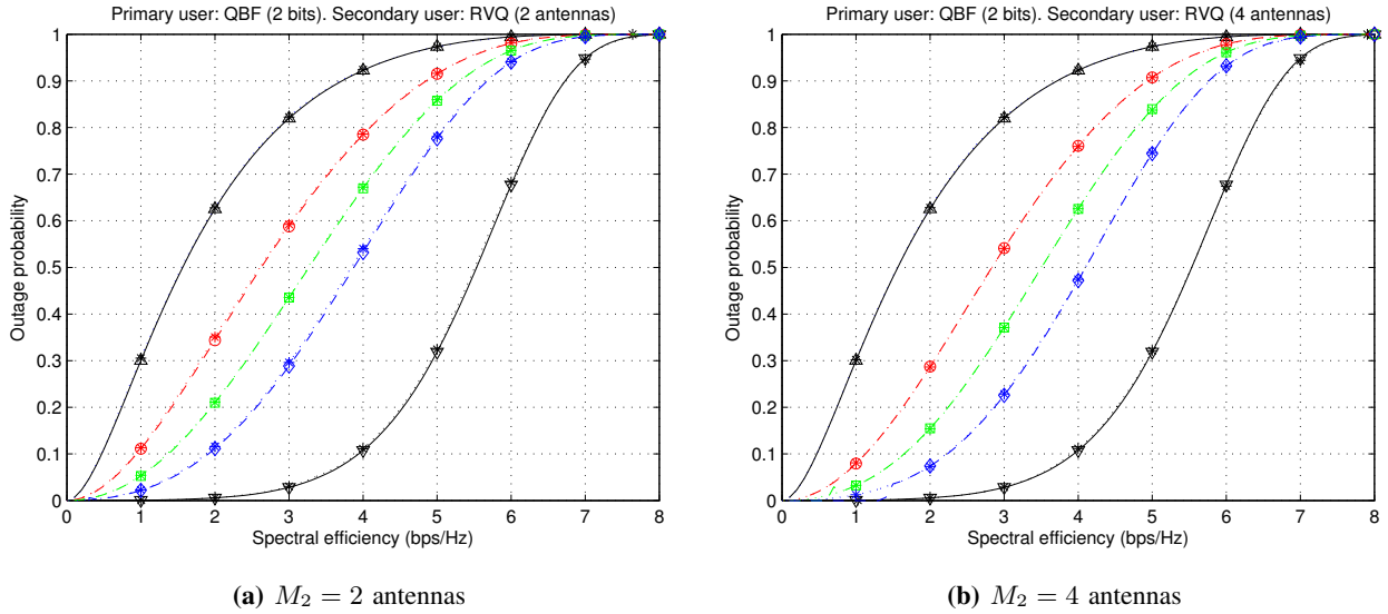
Fig. 2: Rate Cumulative Distribution Function for the primary MS when primary BS applies egoistic TBF with Quantized Cophasing codebook with N_1 = 2 bits, and secondary BS applies egoistic/altruistic TBF with Random Vector Quantization codebook of variable size ( \bar{\gamma}_{1,1} = 15 dB, \bar{\gamma}_{2,1} = 15 dB). Solid lines: secondary BS egoistic (up-pointing triangles), and secondary BS silent (down-pointing triangles). Dashed lines: N_2 = 2 bits (circles), N_2 = 3 bits (squares), and N_2 = 4 bits (diamonds). Simulated values denoted by stars (*).
