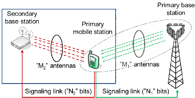
Fig. 1: The downlink system model with co-channel deployment comprises a primary (secondary) BS with M_1 ( M_2 ) transmit antennas, and a primary MS equipped with a single receive antenna. A dedicated low-rate signaling link exists between primary MS and the primary (secondary) BS to convey N_1 ( N_2 ) feedback bits. Primary BS implements egoistic TBF with deterministic codebook design to serve its associated user. Secondary BS mitigate interference at the primary MS using altruistic TBF with randomly generated codebook.
