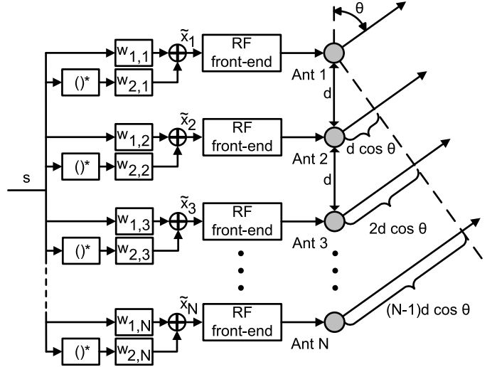
Fig. 2. The conceptual WL digital transmit beamformer.
