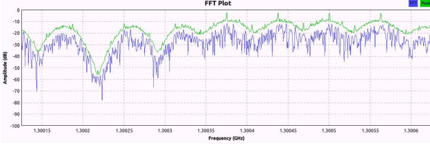
Fig. 2. Primary user sends at multiple bands.
