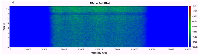
Fig. 4. Sensing results according time at 1.30025GHz.
