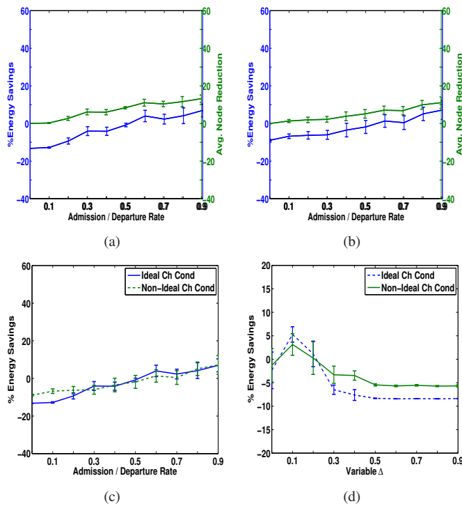
Fig. 3. Greedy Scheme
