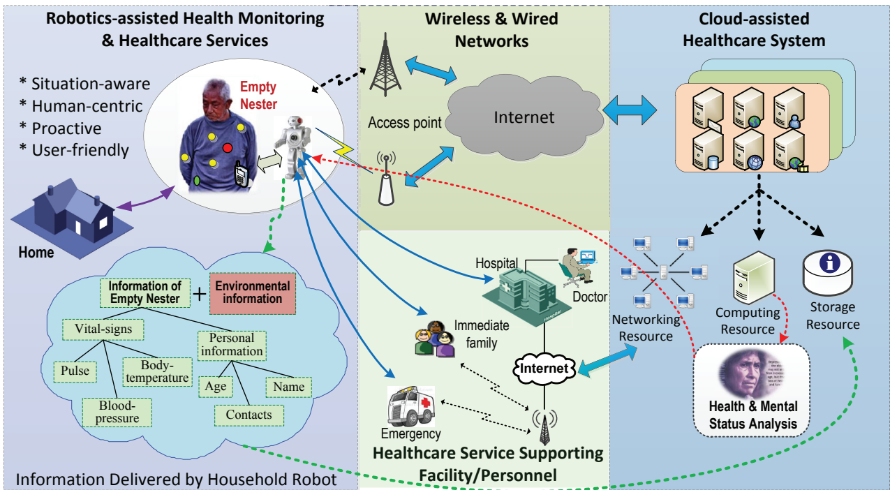
Figure 1: Architecture of ROCHAS
