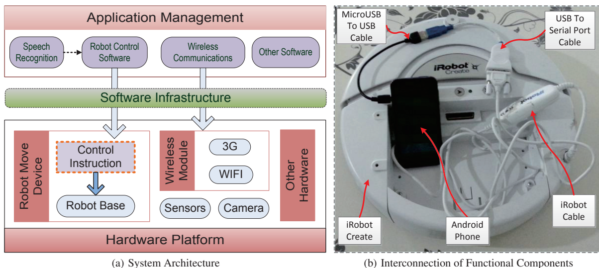
Figure 2: Illustration of The Basic Robot Platform
