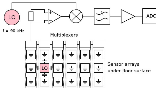
Figure 3 Block diagram of the near field imaging measurement system. The phase sensitive detector takes care of EMI rejection.
