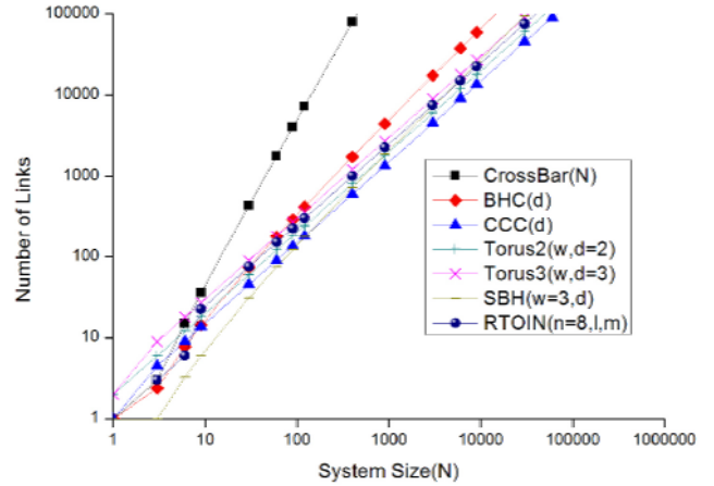
Figure 5: The total number of links with respect to system size for various networks
