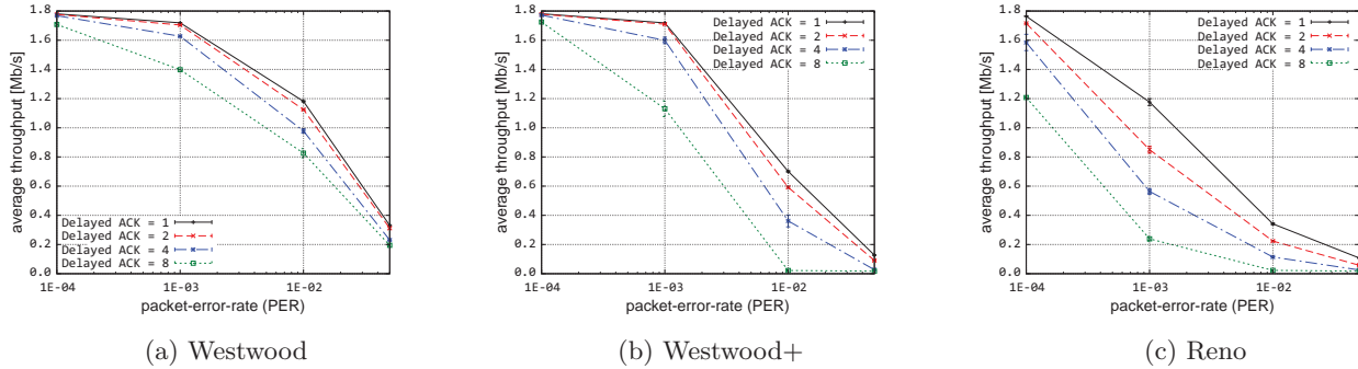
Figure 8: Throughput vs. delayed ACK aggregation count
