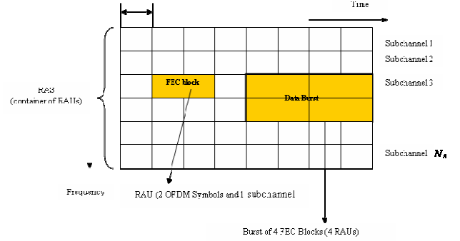
Figure 3. WiMAX Resource Allocation Map (RAM)
