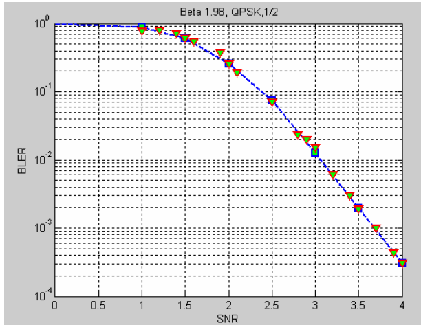
Figure 2. BLER vs. SNR (--=AWGM; ▽= EESM)
