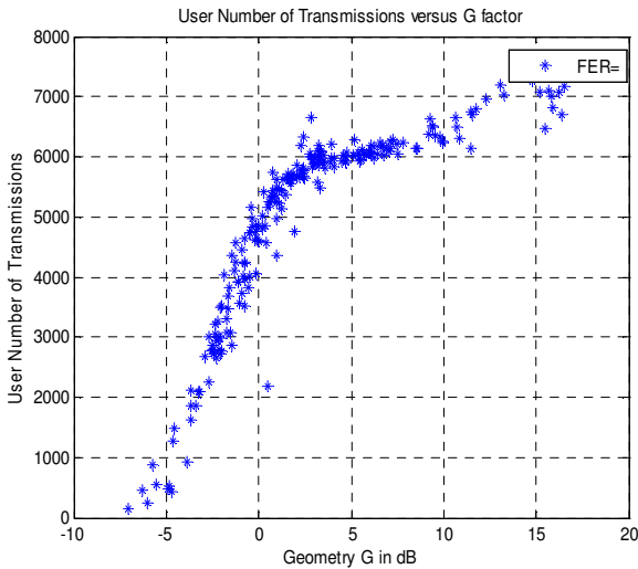
Figure 4. No. of User transmissions vs. Gfactor
