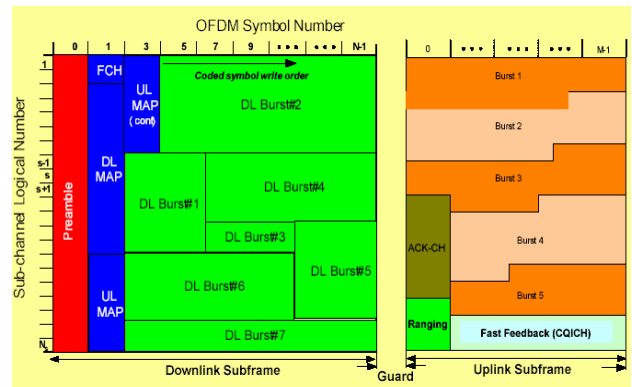
Figure 1. WIMAX Frame Structure
