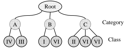
Figure 4. Structure of the HTB tree.
